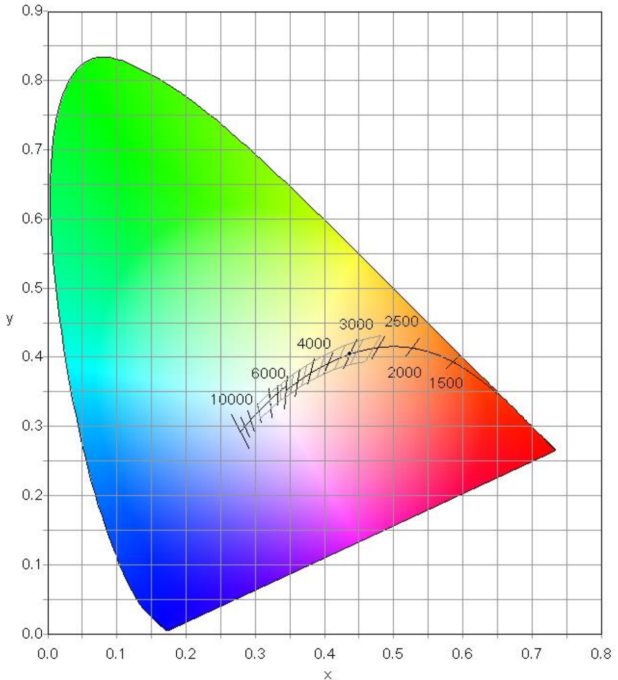
Chart 2: Chromaticity Diagram per Sphere - Spectroradiometer Method
